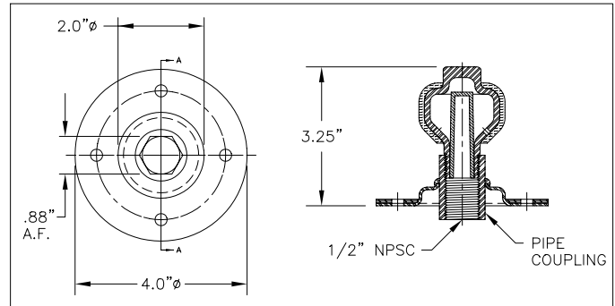
Figure 5: Evasser Dimensions
