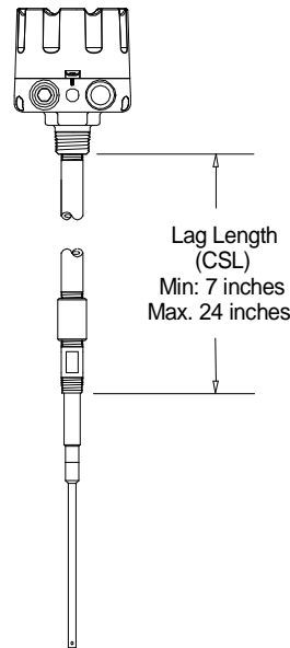
MK-2 or MK-2e Lagged Pipe Extension
