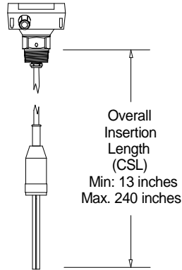
PZP Cable Extension
