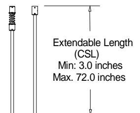
Accessory Probe Extension
