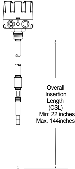
MK-2 or MK-2e Pipe Extension
