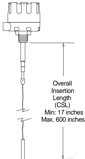
MK-2 or MK-2e Cable Extension
