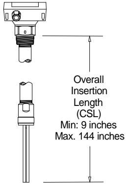
PZP Pipe Extension
