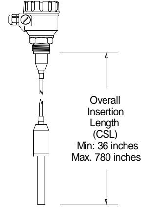
VibraRod Cable Probe Ext.
