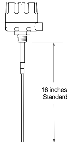
MK-2 or MK-2e Standard
