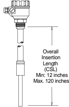
VibraRod Pipe Extension
